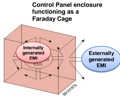
Figure 2. Effective enclosure design provides necessary user access while maximizing the Faraday cage effect when closed, controlling noise inside and outside of a control panel.
